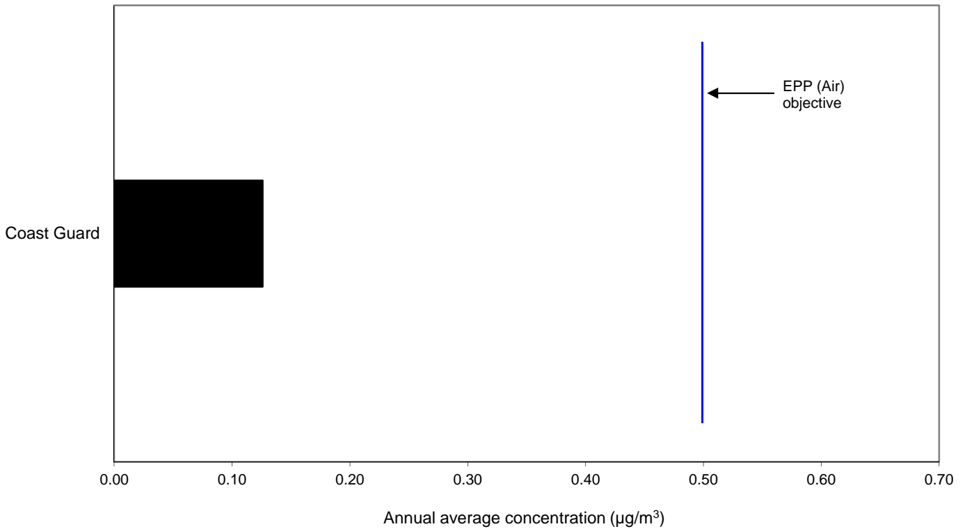
Figure 9. Ambient concentrations of TSP lead (one day in six monitoring) at the Coast Guard site. Annual average concentration ( \mu\text{g}/\text{m}^3 ), October 2014 to September 2015.
