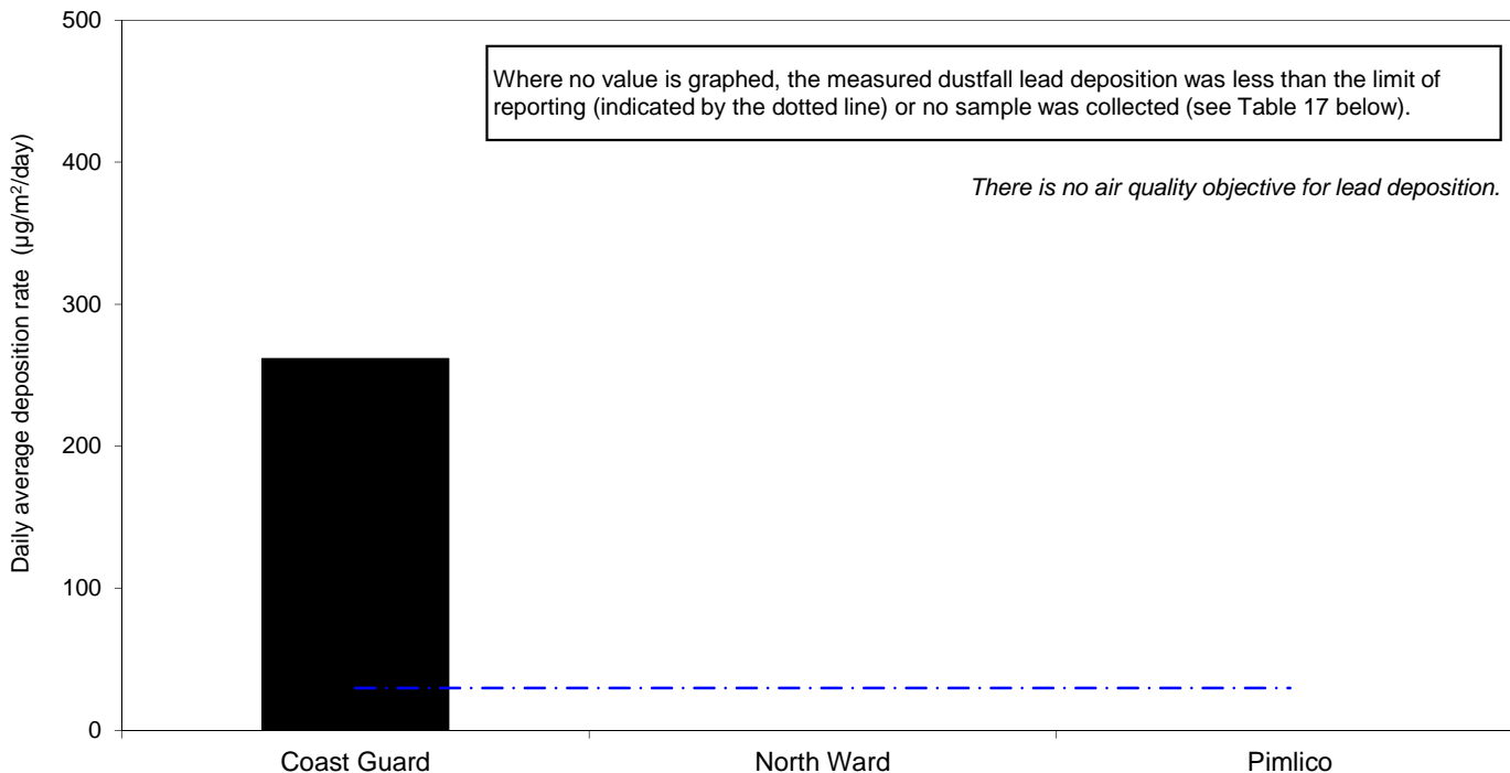
Figure 16. Dustfall lead monitoring at the Coast Guard, North Ward (Warburton Street) and Pimlico sites. Daily average lead deposition rate ( \mu\text{g}/\text{m}^2/\text{day} ) for month of September 2015.
