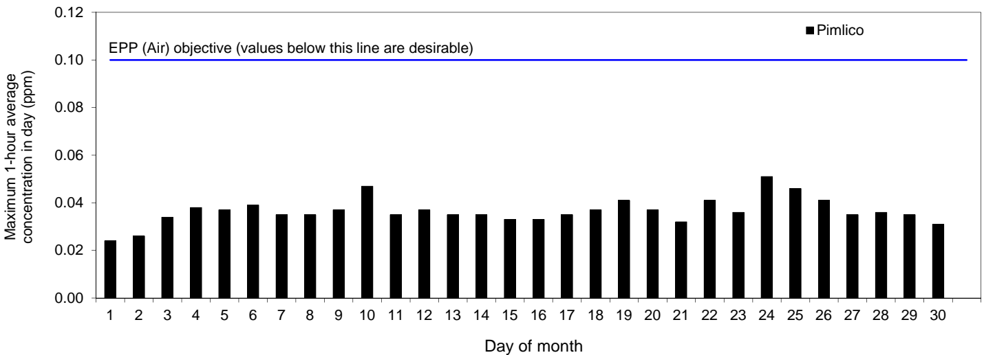
Figure 3. Ambient concentrations of ozone at the Pimlico site. Daily maximum 1-hour average concentrations (ppm), September 2015.
