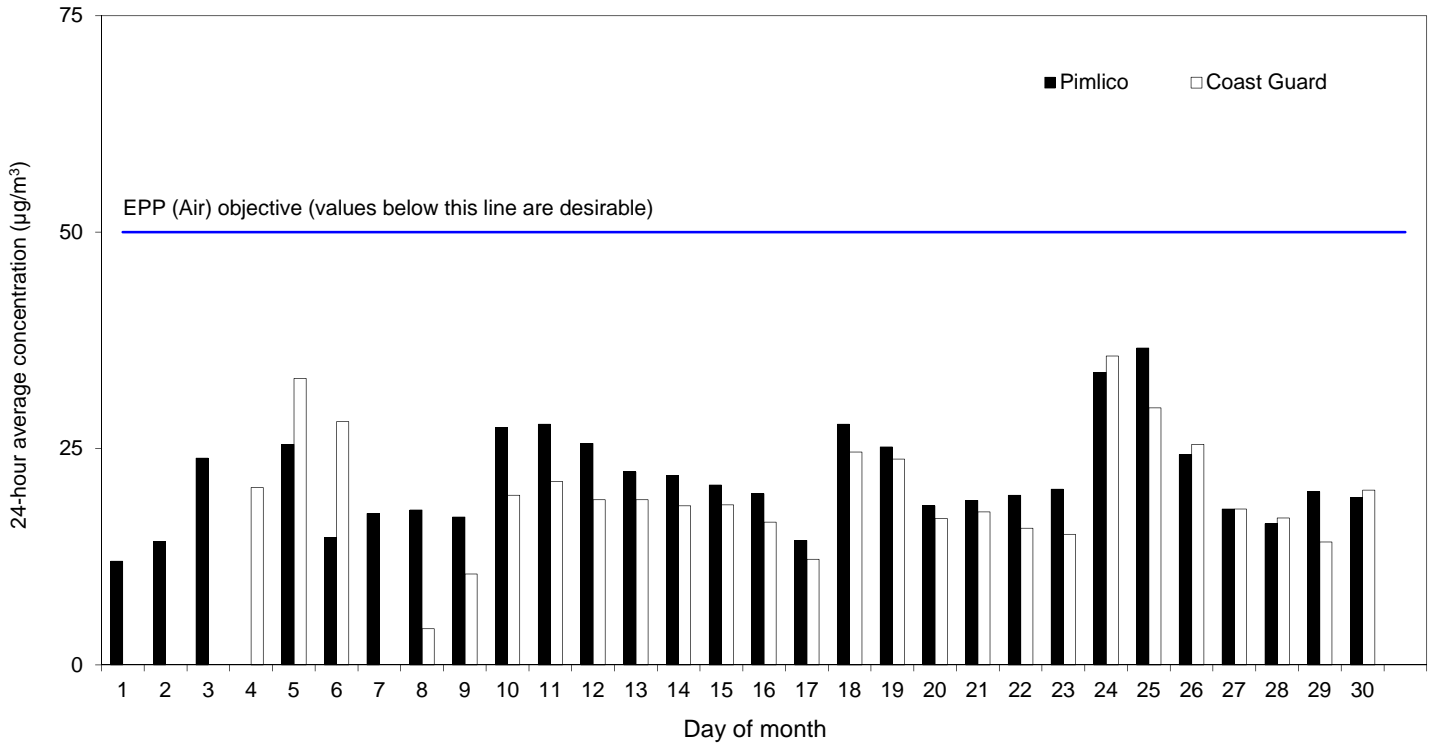
Figure 6. Ambient concentrations of PM 10 at Pimlico and Coast Guard sites. Daily 24-hour average concentrations (µg/m 3 ), September 2015.
