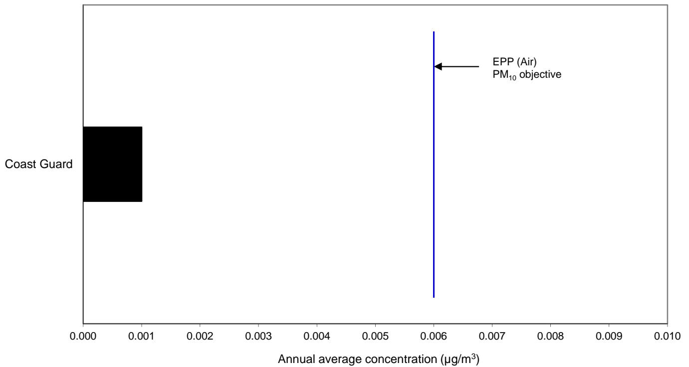
Figure 13. Ambient concentrations of TSP arsenic (one day in six monitoring) at the Coast Guard site. Annual average concentrations ( \mu\text{g}/\text{m}^3 ), October 2014 to September 2015.
