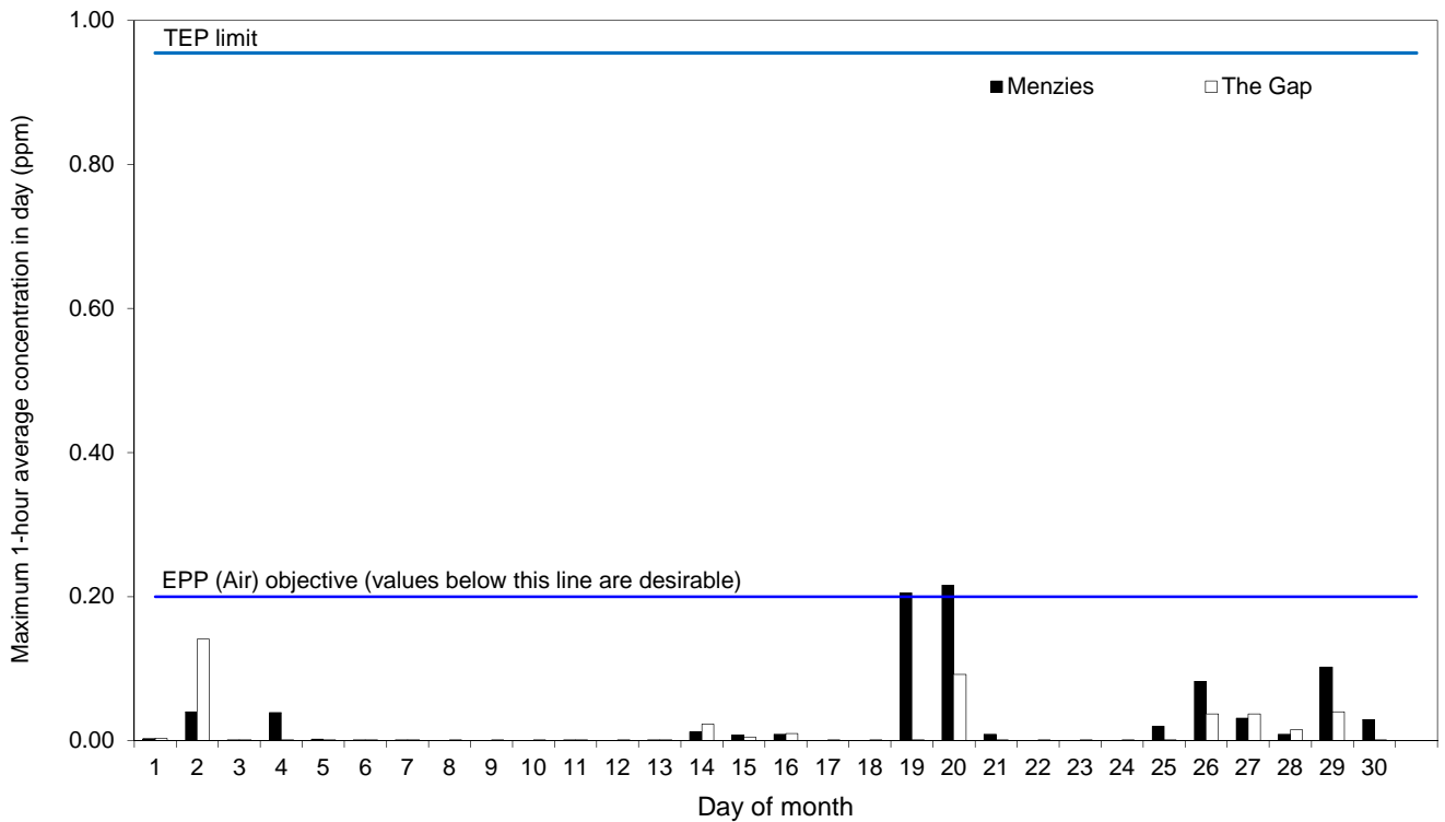
Figure 18. Ambient concentrations of sulfur dioxide at the Menzies and The Gap sites. Daily maximum 1-hour average concentrations (ppm), September 2015.
