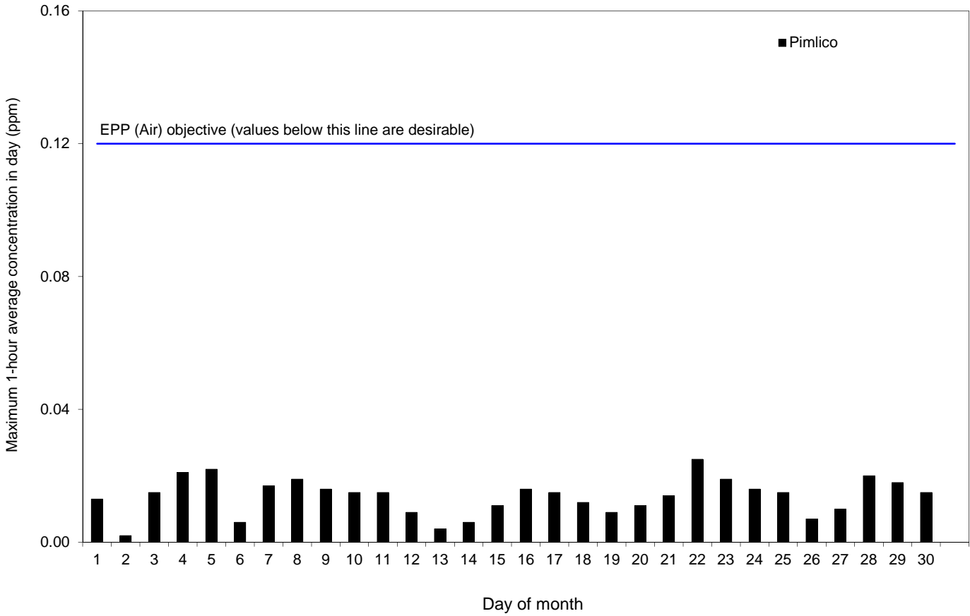
Figure 1. Ambient concentrations of nitrogen dioxide at the Pimlico site. Daily maximum 1-hour average concentrations (ppm), September 2015.
