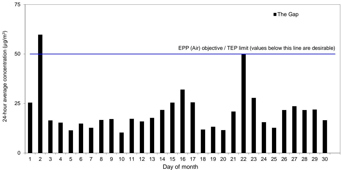
Figure 19. Ambient concentrations of PM 10 at The Gap site. Daily 24-hour average concentrations (µg/m 3 ), September 2015.
