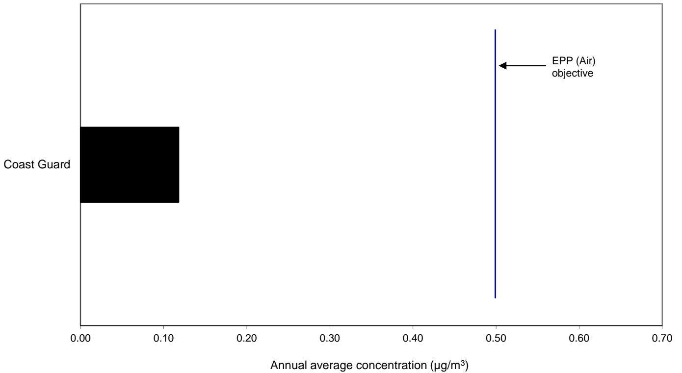
Figure 9. Ambient concentrations of TSP lead (one day in six monitoring) at the Coast Guard site. Annual average concentration ( \mu\text{g}/\text{m}^3 ), November 2014 to October 2015.
