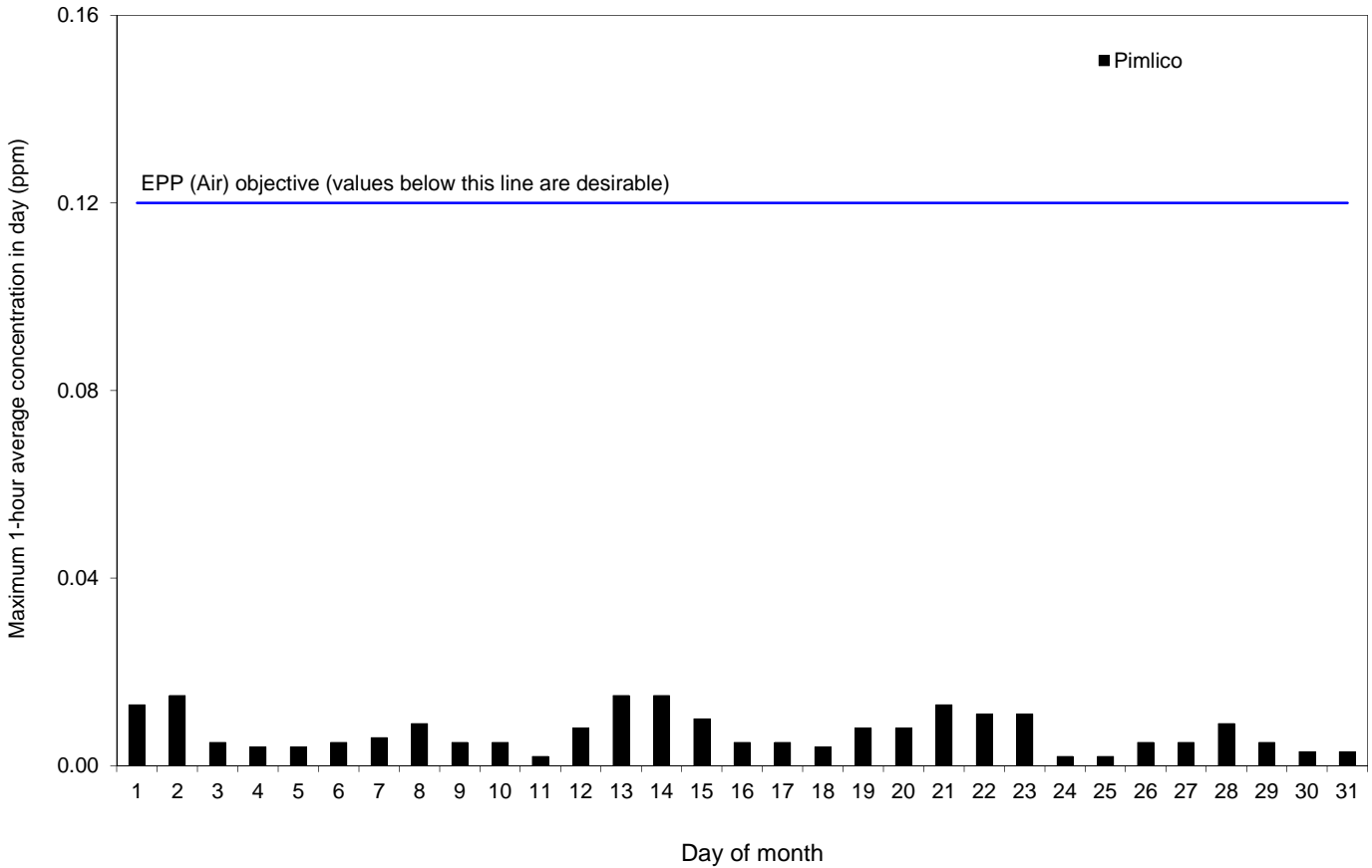
Figure 1. Ambient concentrations of nitrogen dioxide at the Pimlico site. Daily maximum 1-hour average concentrations (ppm), October 2015.
