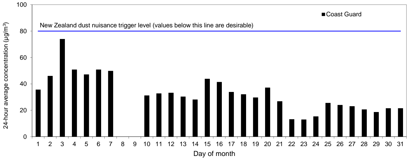
Figure 8. Ambient concentrations of TSP (one day in six monitoring) at the Coast Guard site. 24-hour average concentrations ( \mu\text{g}/\text{m}^3 ), October 2015.
