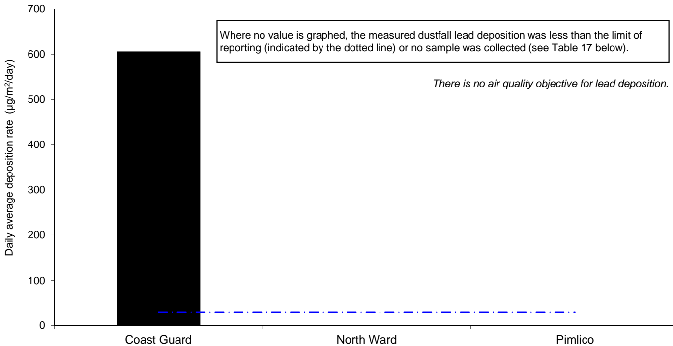
Figure 16. Dustfall lead monitoring at the Coast Guard, North Ward (Warburton Street) and Pimlico sites. Daily average lead deposition rate ( \mu\text{g}/\text{m}^2/\text{day} ) for month of October 2015.
