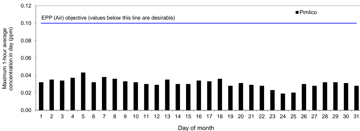
Figure 3. Ambient concentrations of ozone at the Pimlico site. Daily maximum 1-hour average concentrations (ppm), October 2015.
