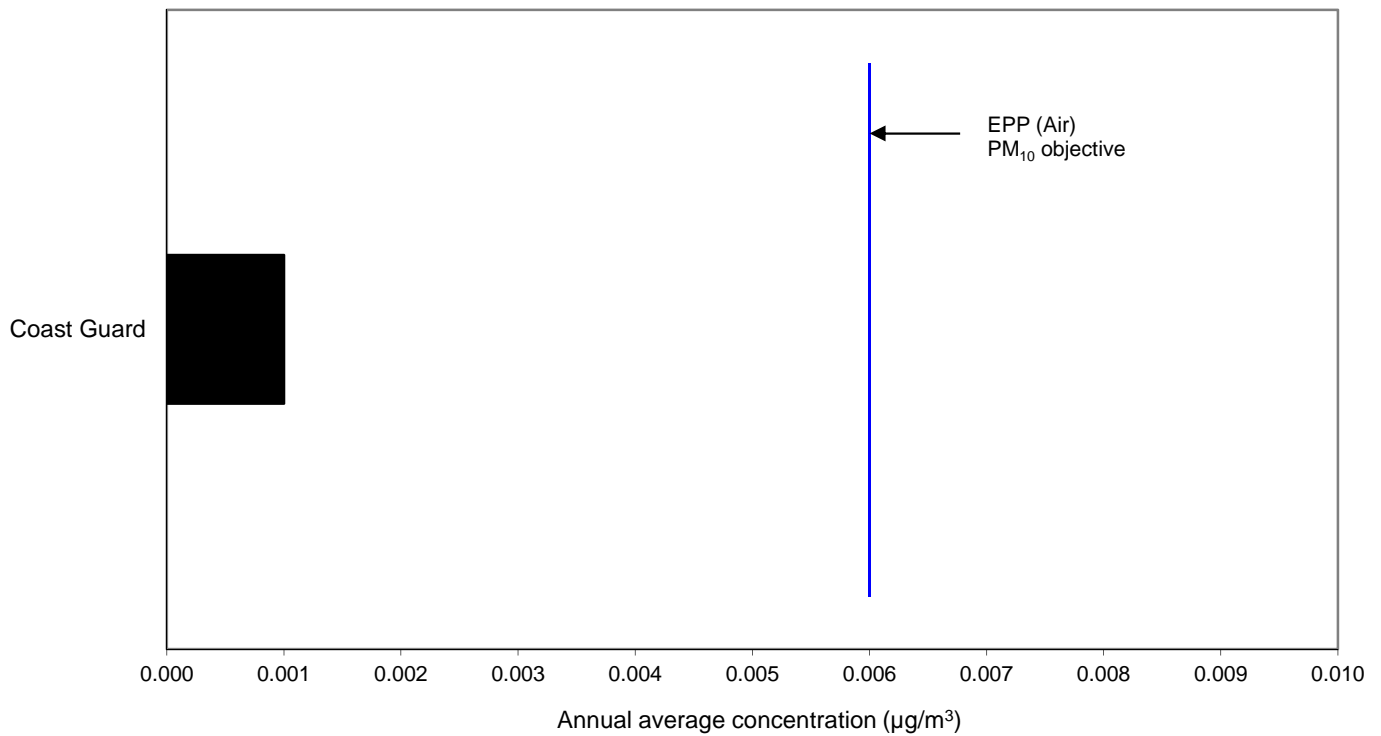
Figure 13. Ambient concentrations of TSP arsenic (one day in six monitoring) at the Coast Guard site. Annual average concentrations ( \mu\text{g}/\text{m}^3 ), November 2014 to October 2015.
