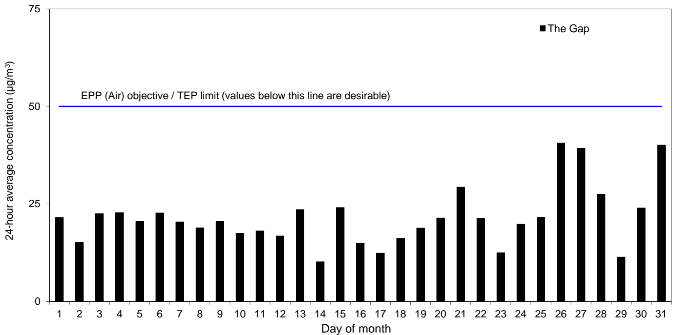
Figure 19. Ambient concentrations of PM 10 at The Gap site. Daily 24-hour average concentrations (µg/m 3 ), October 2015.
