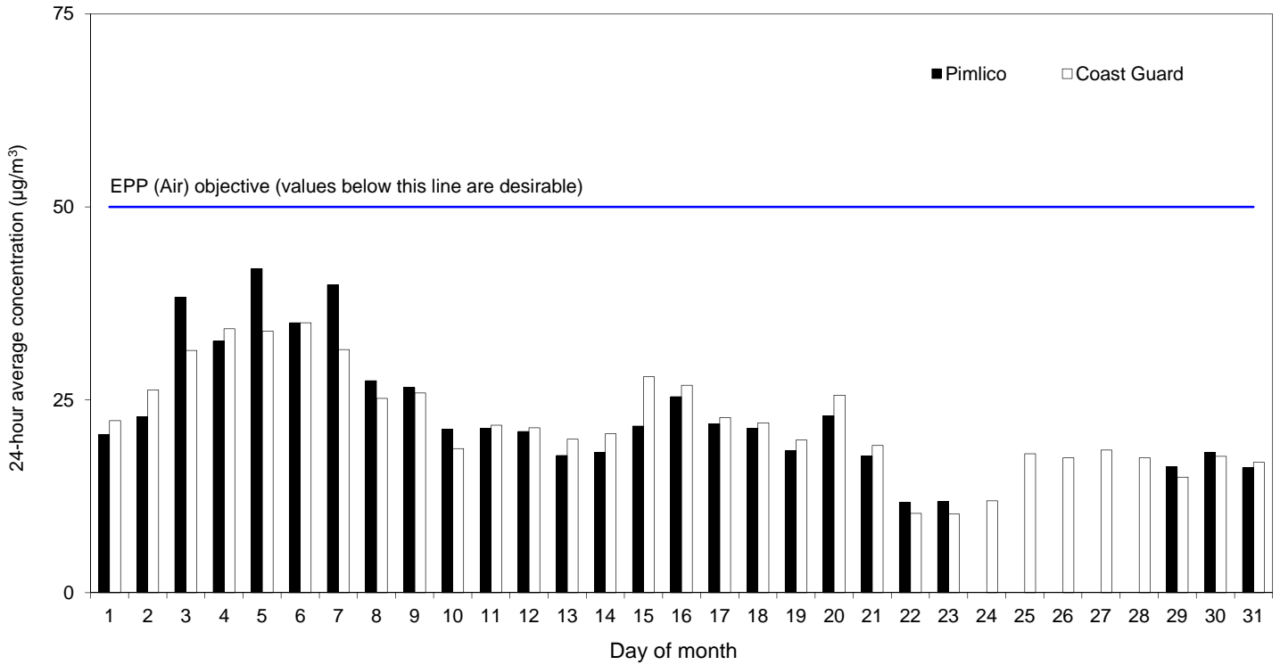
Figure 6. Ambient concentrations of PM 10 at Pimlico and Coast Guard sites. Daily 24-hour average concentrations (µg/m 3 ), October 2015.
