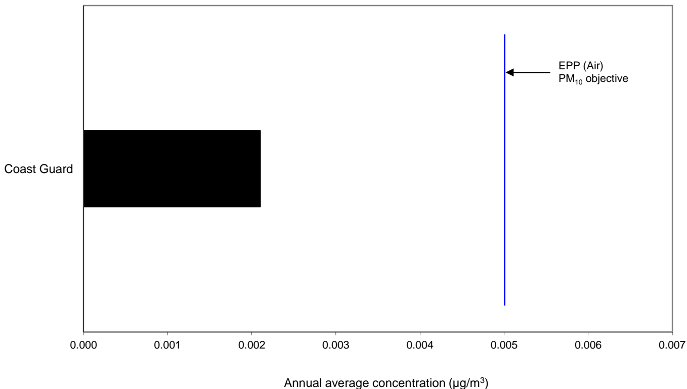
Figure 14. Ambient concentrations of TSP cadmium (one day in six monitoring) at the Coast Guard site. Annual average concentrations ( \mu\text{g}/\text{m}^3 ), November 2014 to October 2015.
