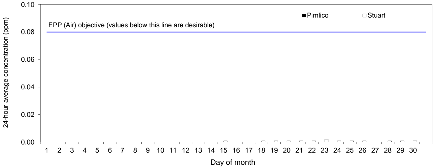
Figure 5. Ambient concentrations of sulfur dioxide at Pimlico and Stuart sites. Daily maximum 1-hour average concentrations (ppm), November 2015.
