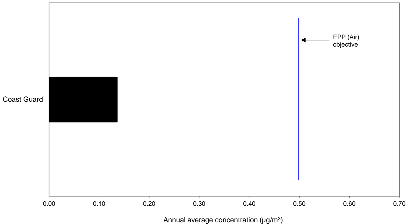
Figure 9. Ambient concentrations of TSP lead (one day in six monitoring) at the Coast Guard site. Annual average concentration ( \mu\text{g}/\text{m}^3 ), December 2014 to November 2015.
