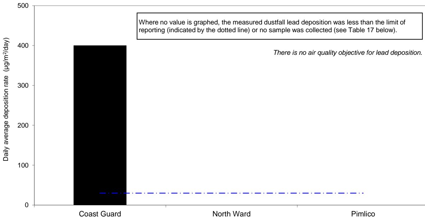
Figure 16. Dustfall lead monitoring at the Coast Guard, North Ward (Warburton Street) and Pimlico sites. Daily average lead deposition rate ( \mu\text{g}/\text{m}^2/\text{day} ) for month of November 2015.
