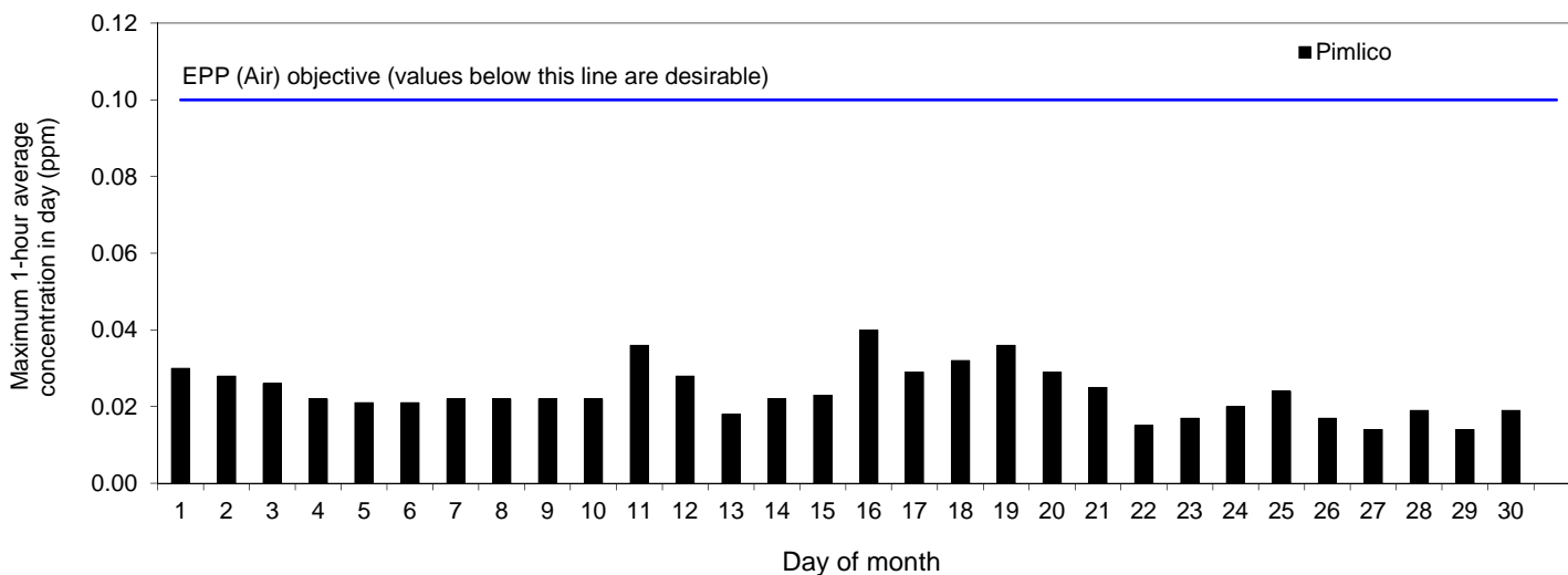
Figure 3. Ambient concentrations of ozone at the Pimlico site. Daily maximum 1-hour average concentrations (ppm), November 2015.
