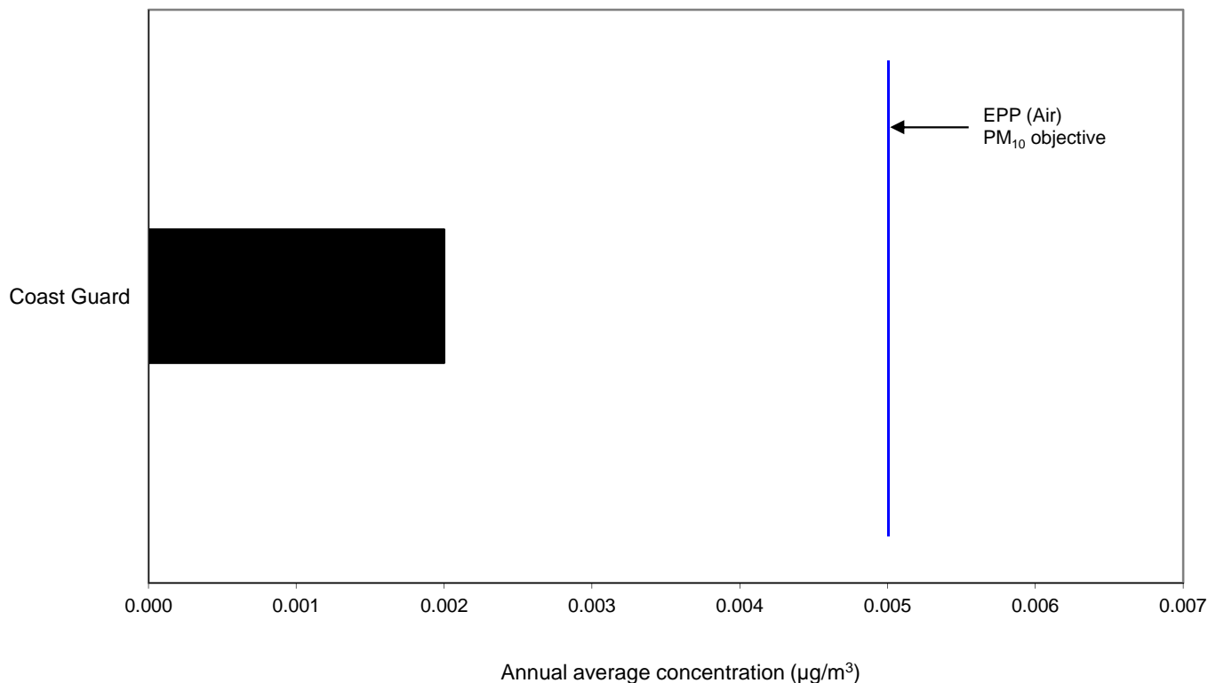
Figure 14. Ambient concentrations of TSP cadmium (one day in six monitoring) at the Coast Guard site. Annual average concentrations ( \mu\text{g}/\text{m}^3 ), December 2014 to November 2015.
