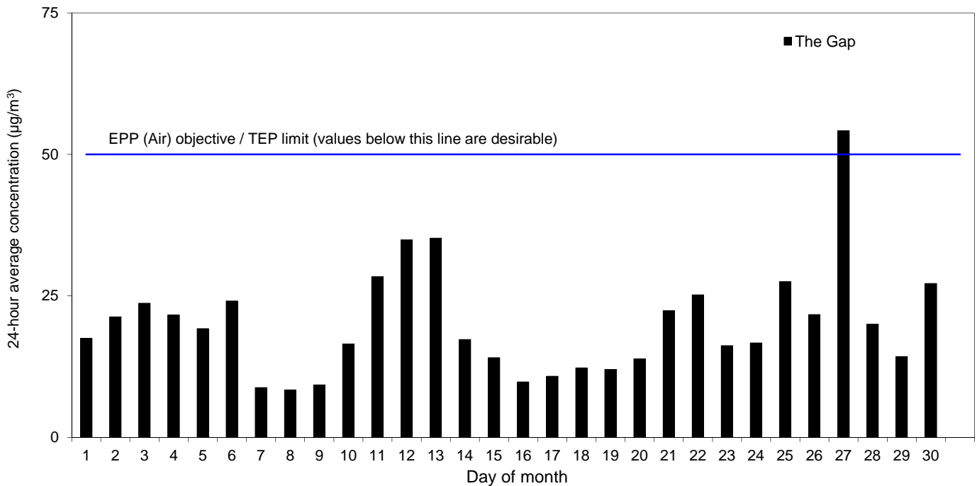
Figure 19. Ambient concentrations of PM 10 at The Gap site. Daily 24-hour average concentrations (µg/m 3 ), November 2015.
