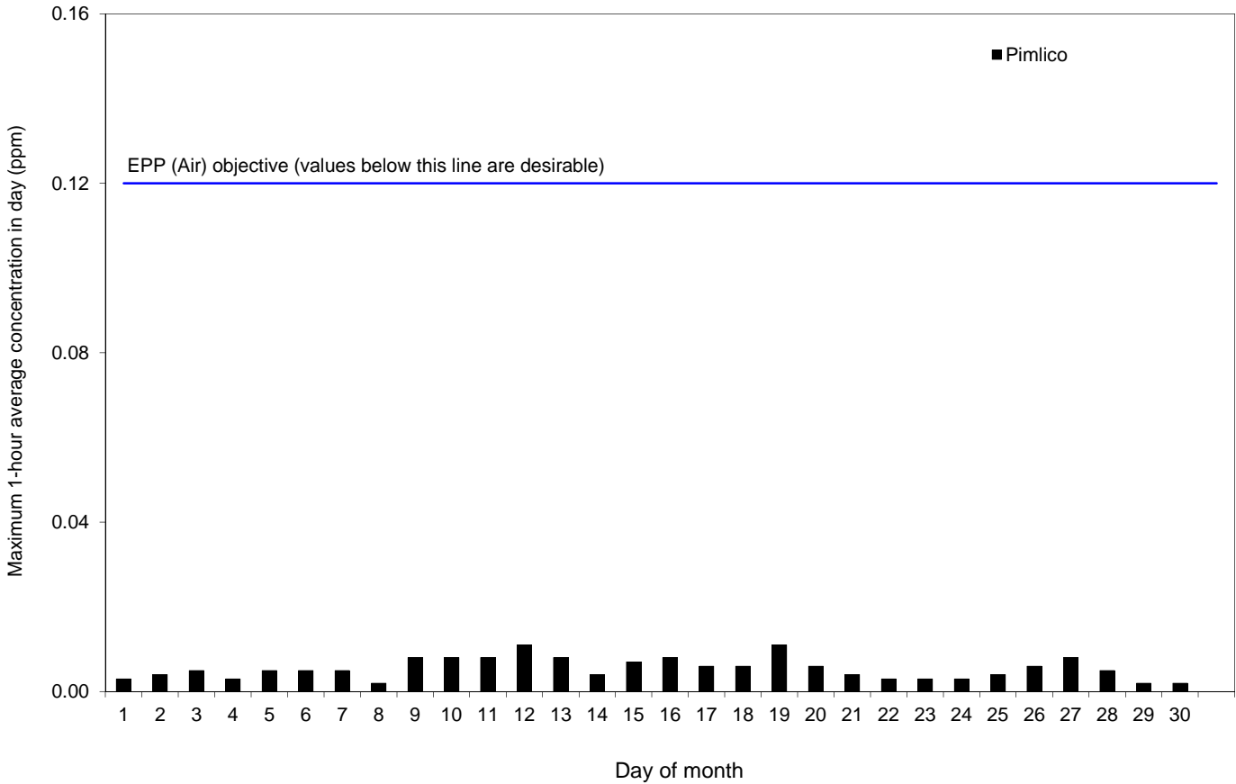
Figure 1. Ambient concentrations of nitrogen dioxide at the Pimlico site. Daily maximum 1-hour average concentrations (ppm), November 2015.
