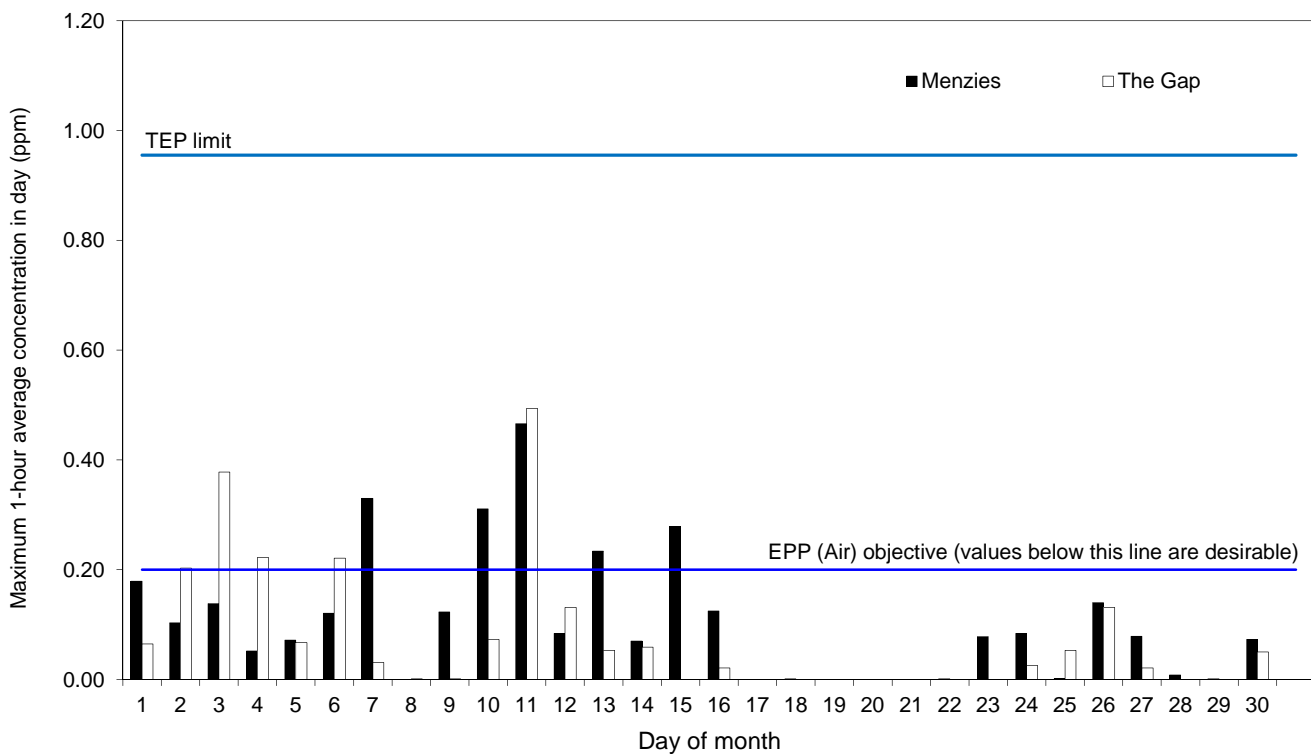
Figure 18. Ambient concentrations of sulfur dioxide at the Menzies and The Gap sites. Daily maximum 1-hour average concentrations (ppm), November 2015.
