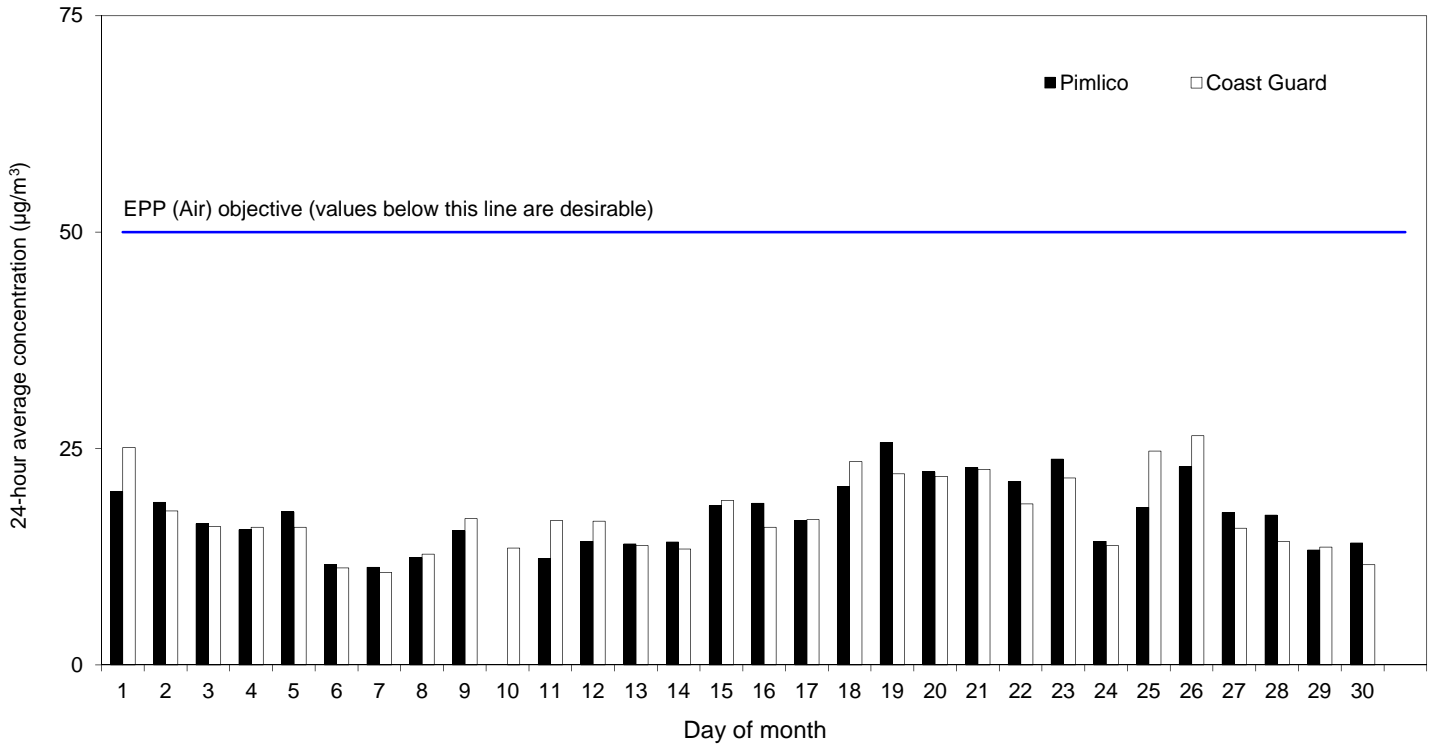
Figure 6. Ambient concentrations of PM 10 at Pimlico and Coast Guard sites. Daily 24-hour average concentrations (µg/m 3 ), November 2015.
