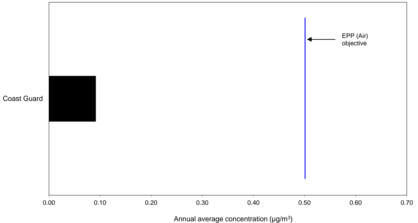
Figure 6. Ambient concentrations of TSP lead (one day in six monitoring) at the Coast Guard site. Annual average concentration ( \mu\text{g}/\text{m}^3 ), May 2015 to April 2016.
