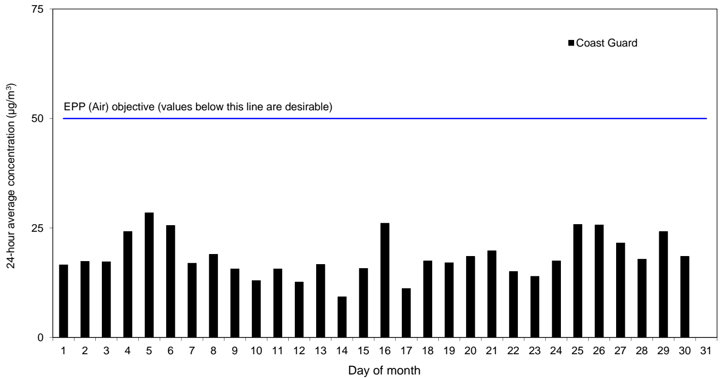
Figure 3. Ambient concentrations of PM 10 at the Coast Guard site. Daily 24-hour average concentrations (µg/m 3 ), April 2016.
