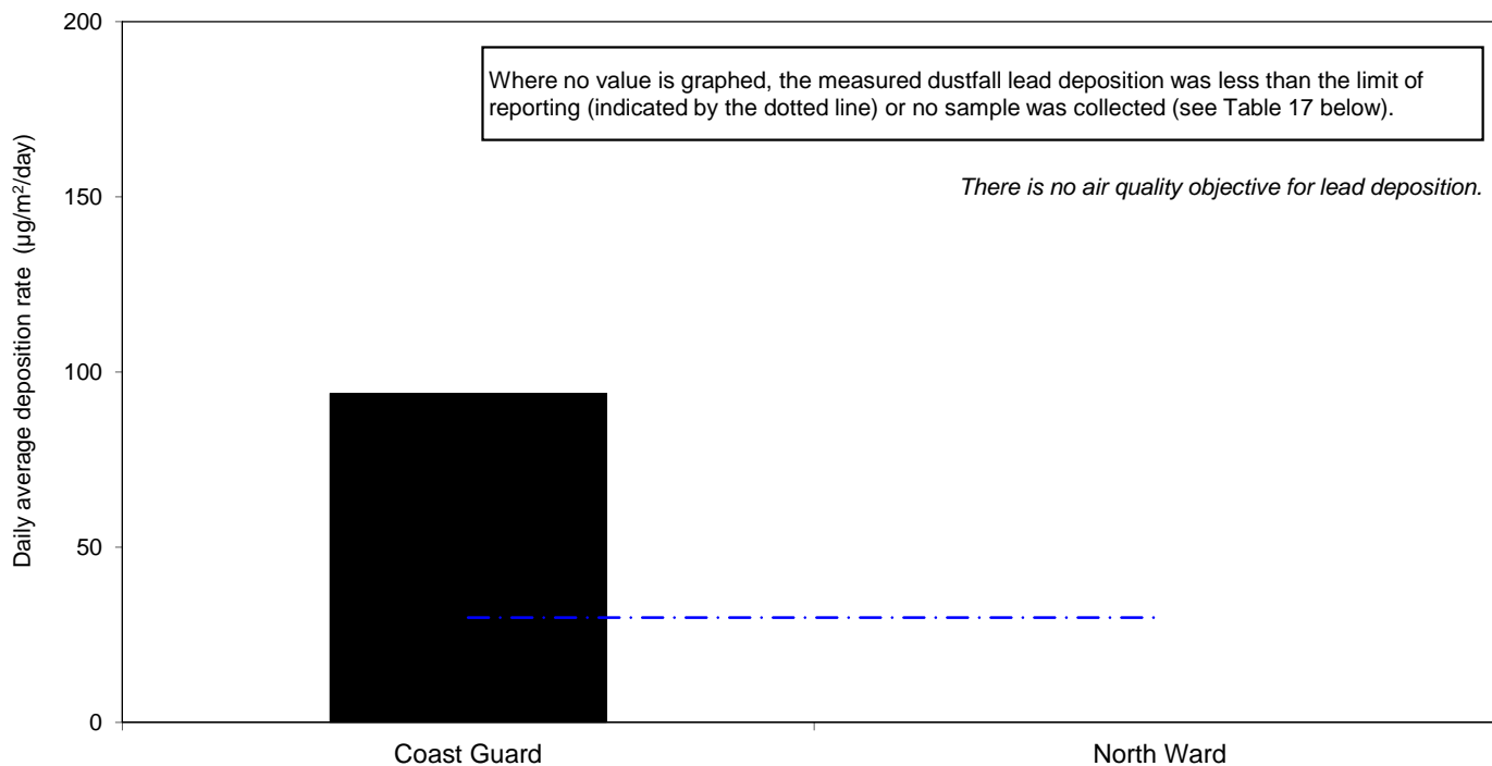
Figure 13. Dustfall lead monitoring at the Coast Guard and North Ward (Warburton Street) sites. Daily average lead deposition rate ( \mu\text{g}/\text{m}^2/\text{day} ) for month of April 2016.
