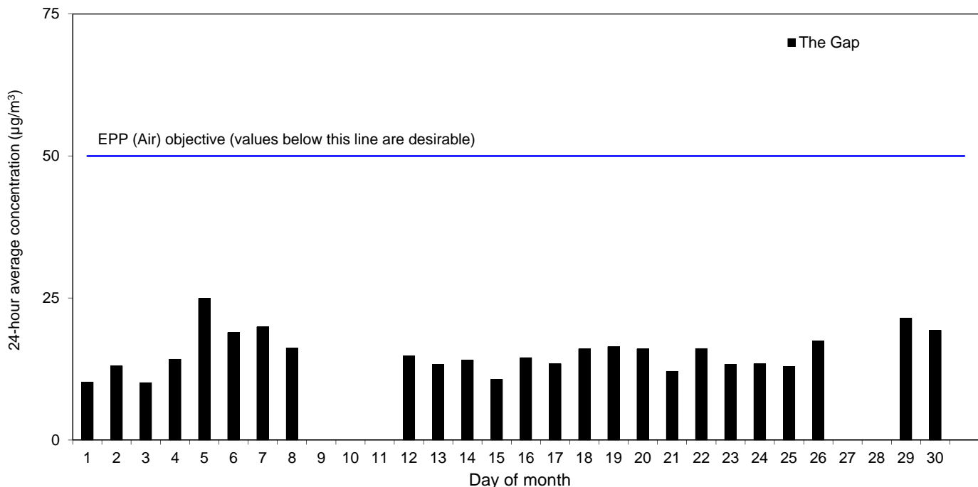
Figure 16. Ambient concentrations of PM 10 at The Gap site. Daily 24-hour average concentrations (µg/m 3 ), April 2016.
