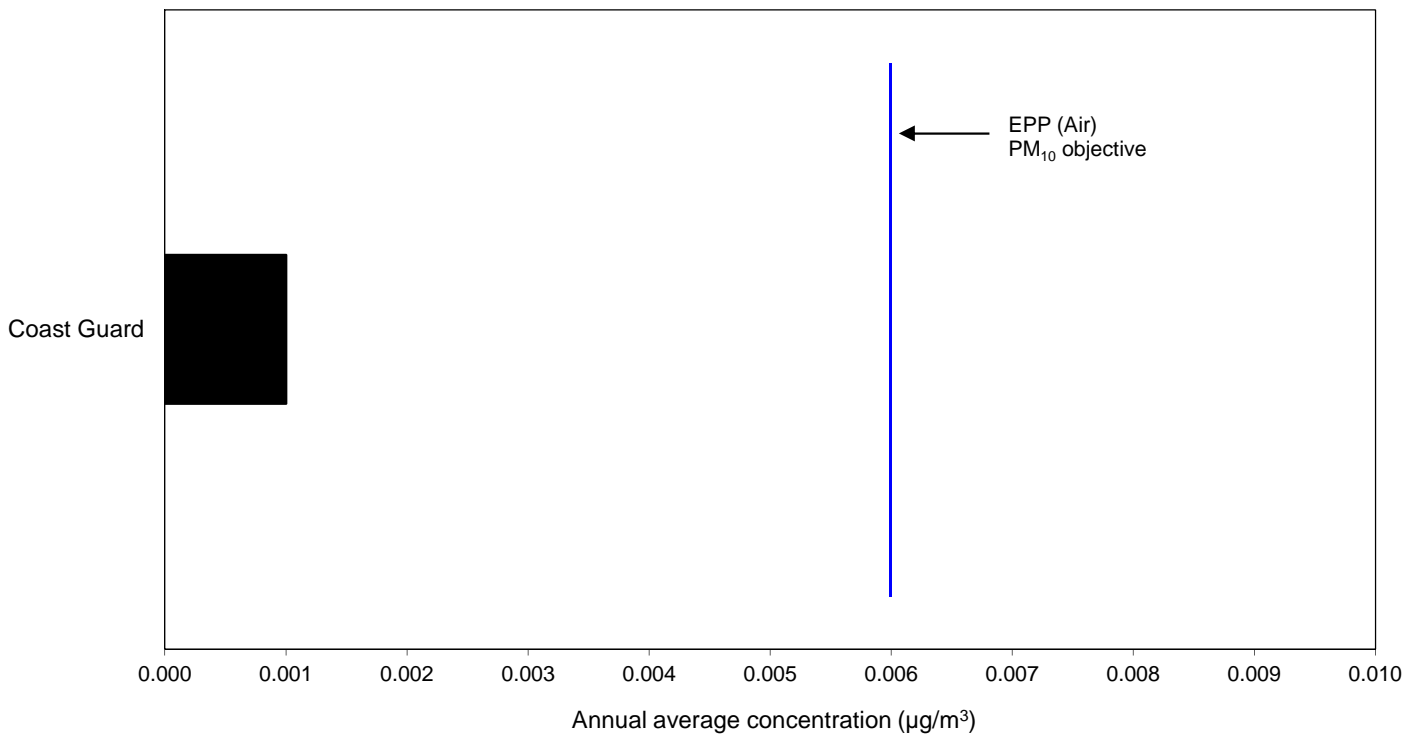
Figure 10. Ambient concentrations of TSP arsenic (one day in six monitoring) at the Coast Guard site. Annual average concentrations ( \mu\text{g}/\text{m}^3 ), May 2015 to April 2016.
