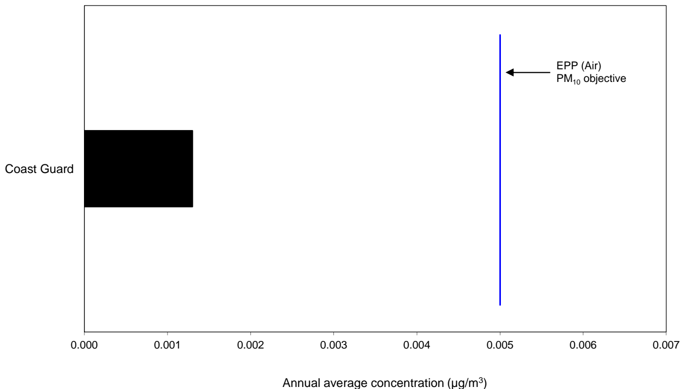
Figure 11. Ambient concentrations of TSP cadmium (one day in six monitoring) at the Coast Guard site. Annual average concentrations ( \mu\text{g}/\text{m}^3 ), May 2015 to April 2016.
