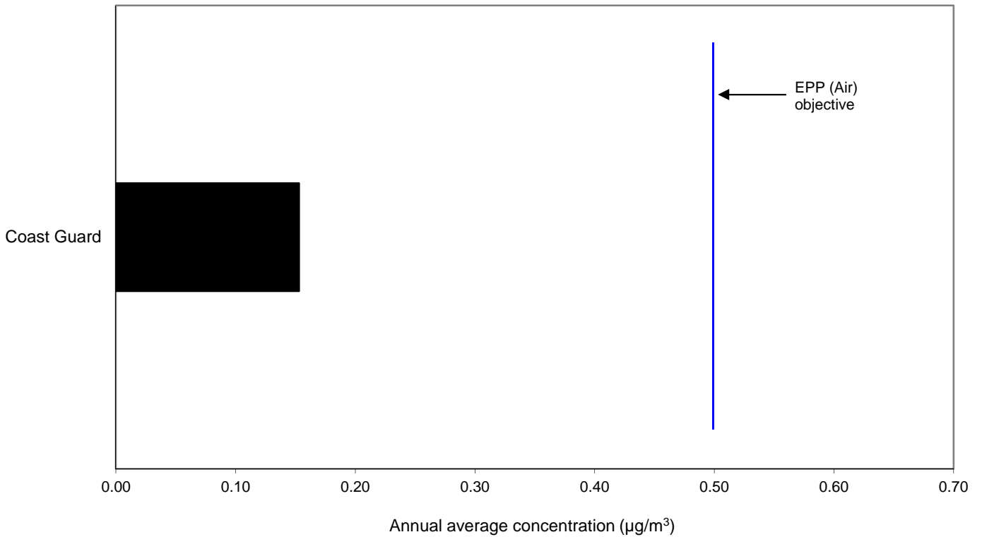
Figure 9. Ambient concentrations of TSP lead (one day in six monitoring) at the Coast Guard site. Annual average concentration ( \mu\text{g}/\text{m}^3 ), June 2014 to May 2015.
