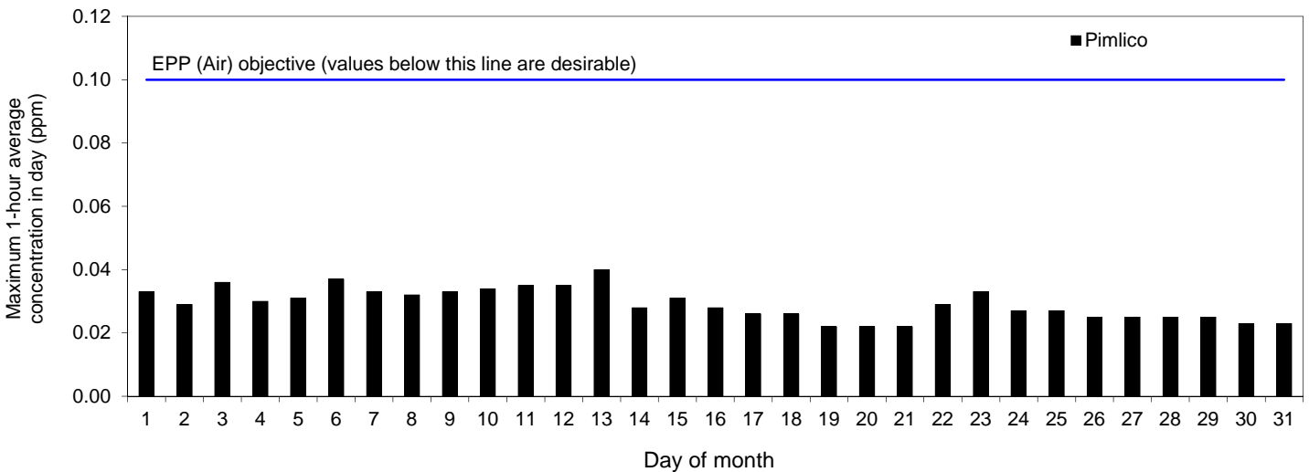
Figure 3. Ambient concentrations of ozone at the Pimlico site. Daily maximum 1-hour average concentrations (ppm), May 2015.
