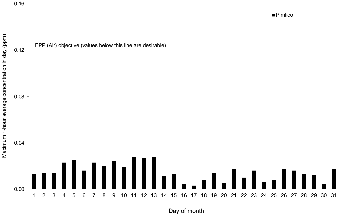
Figure 1. Ambient concentrations of nitrogen dioxide at the Pimlico site. Daily maximum 1-hour average concentrations (ppm), May 2015.
