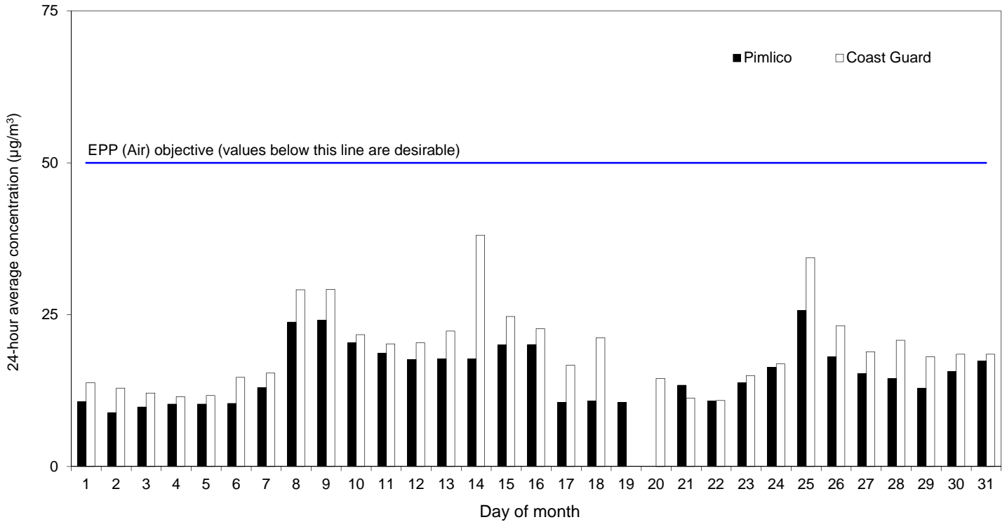
Figure 6. Ambient concentrations of PM 10 at Pimlico and Coast Guard sites. Daily 24-hour average concentrations (µg/m 3 ), May 2015.
