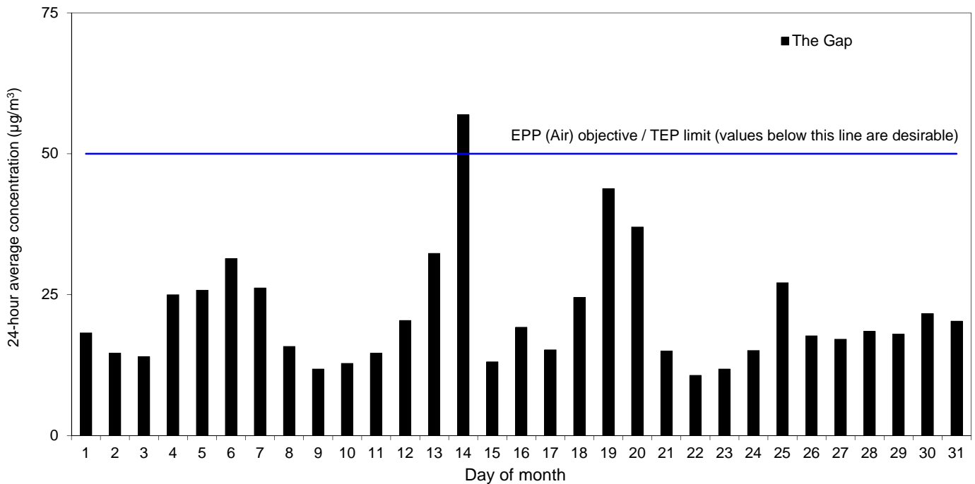
Figure 19. Ambient concentrations of PM 10 at The Gap site. Daily 24-hour average concentrations (µg/m 3 ), May 2015.
