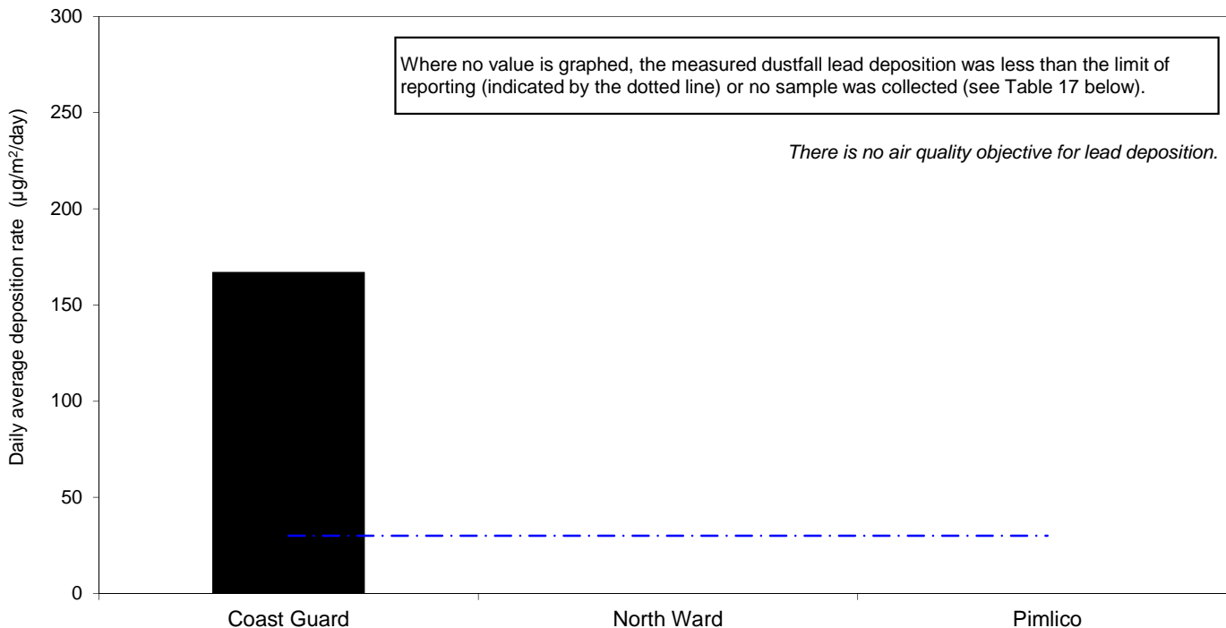
Figure 16. Dustfall lead monitoring at the Coast Guard, North Ward (Warburton Street) and Pimlico sites. Daily average lead deposition rate ( \mu\text{g}/\text{m}^2/\text{day} ) for month of May 2015.
